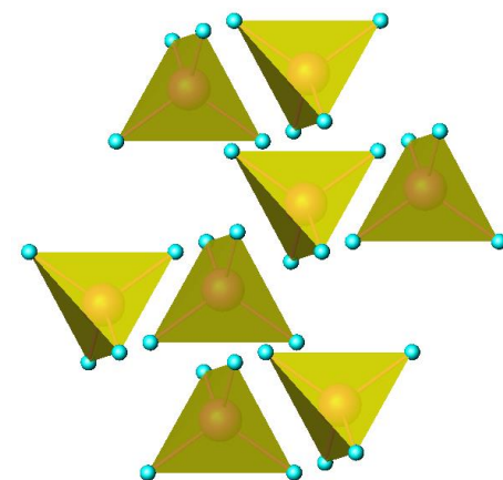
PtCl 4
