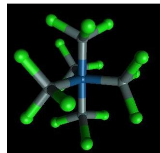
[\text{Pt}(\text{SnCl}_3)_5]^{3-}
