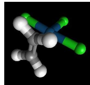
[\text{PtCl}_3(\text{C}_2\text{H}_4)]^-
