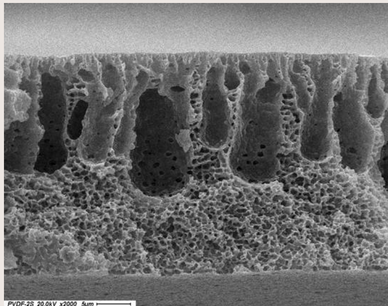
PVDF-2S 20.0kV x2000 5um
