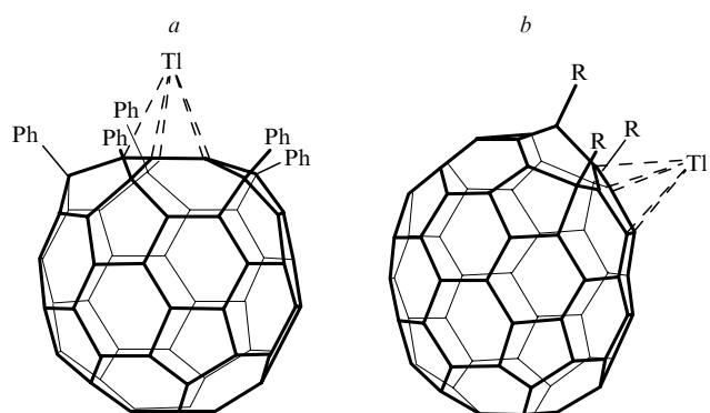
Figure 28. Examples of the \eta^5 -coordination fullerene–metal. ( a ) C 60 Ph 5 Tl · 2.5 THF, Tl–C = 2.83–2.89 Å (see Ref. 238), ( b ) C 70 (C 6 H 4 CF 3 ) 3 Tl · C 6 H 4 Cl 2 , Tl–C = 2.84–3.08 Å (R = p -C 6 H 4 CF 3 ). 240
