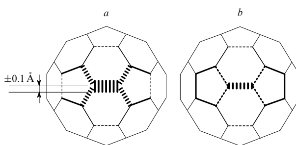
Figure 25. The elongation (dashed lines) and shortening (solid lines) of bonds in the fullerene molecule upon \sigma - (a) and \pi -addition (b). The magnitude of the bond length changes is proportional to the line width (the scale is shown).
