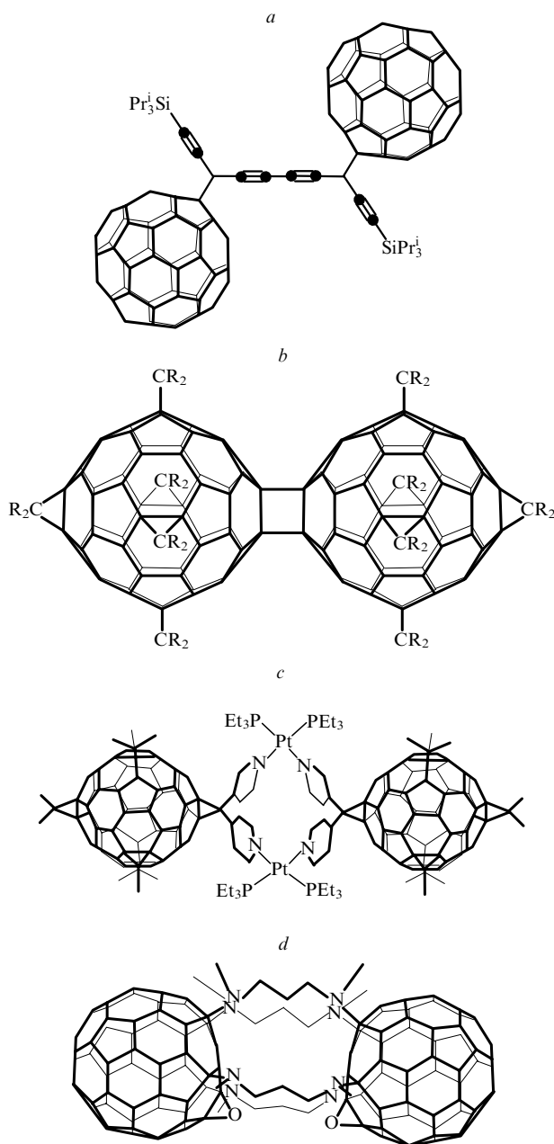
Figure 23. The structures of molecules containing two C_{60} moieties; (a) 1,4-bis[(1,2-dihydro-61-[(triisopropylsilyl)ethynyl]-1,2-methano- C_{60} -fullerene-61-yl]buta-1,3-diyne, 219 (b) bis[decakis(ethoxycarbonyl)pentacyclopropane(1,9:16,17:44,45:52,60)- C_{60} -fullerenediyl], 220 (c) bis[ \mu^2 -66,66-bis(4-pyridyl)-1,2:18,36:22,23:27,45:31,32:55,56-hexakis(methano)- C_{60} -fullerene-61,61,62,62,63,63,64,64,65,65-decakis(ethylcarbonate)- N,N' ]bis(triphenylphosphino) platinum(II), 221 (d) tetrakis( N,N' -dimehylpropanediamine- N,N' )bis(epoxy- C_{60} -fullerene). 222
