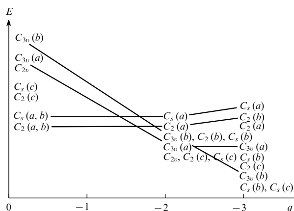
Figure 2. The relative stabilities of different geometrical isomers of C n q- (see Ref. 19).
