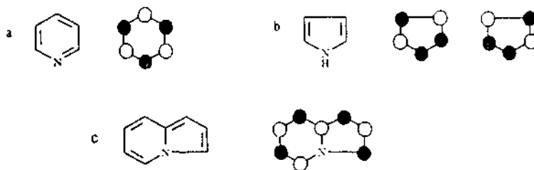
Scheme 9. Distribution of polarity in the skeleta of alternant and nonalternant heterocycles. (The donating centers are black, and the accepting centers are white.)
