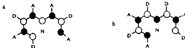
Scheme 10. Normal (a) and reverse (b) alternation of the chain in bridged azoloazines.
