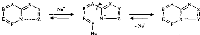
Scheme 3. Dimroth rearrangement in the series of azaindolizines with 5 → 4 exo cleavage.
