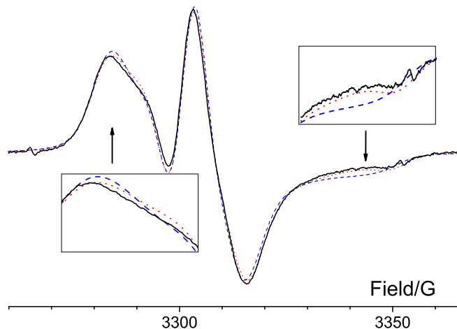
Fig. 7. One experimental spectrum from the set of spectra shown in Fig. 5a (solid line) and spectra calculated in the course of joint fitting of whole set with use of expansion ranks 2 (dashed line) and 4 (dotted line) within OD approach.
