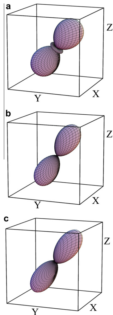
Fig. 11. Orientation distribution functions of R2 probe in liquid crystal 5CB; (a) 77 K, ODF has negative part, (b) 77 K, ODF is positive in all angular space, (c) 293 K, ODF determined using OP approach.
